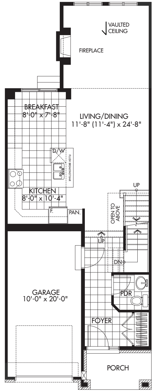
GROUND FLOOR
