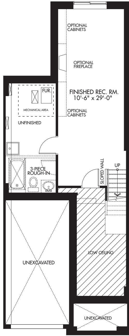
BASEMENT
